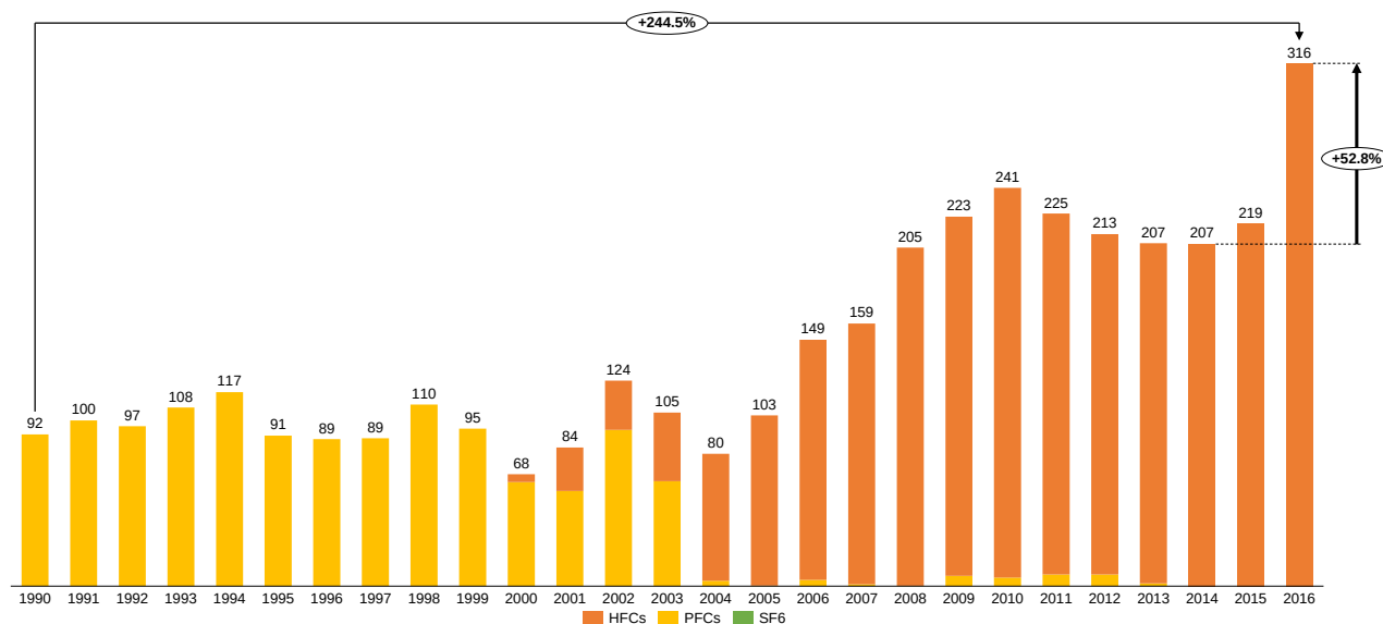
Figure 3-7: Emissions of F-gases (in Gg CO 2 -eq)
