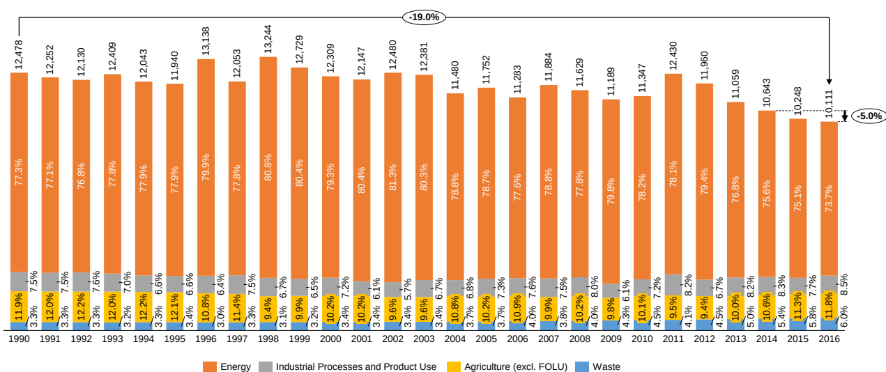
Figure 0-2: Total GHG emissions by sector, excluding FOLU sector (in Gg CO 2 -eq)
