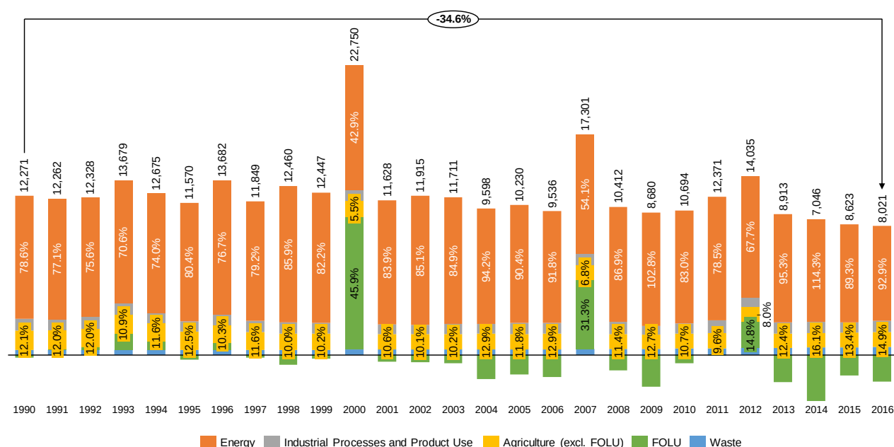
Figure 0-1: GHG emissions and removals by sector (in Gg CO 2 -eq)
