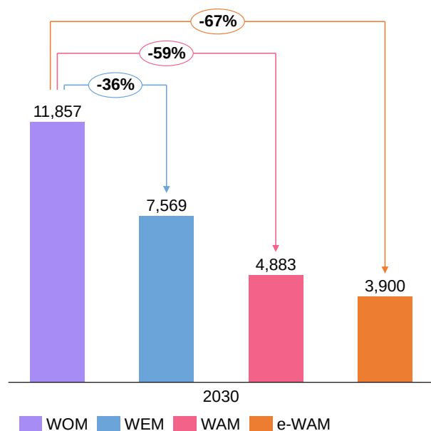
Figure 4-14: Comparison of total GHG emissions from all sectors in WOM, WEM, WAM and e- WAM scenarios, 2030 (in Gg CO 2 -eq)
