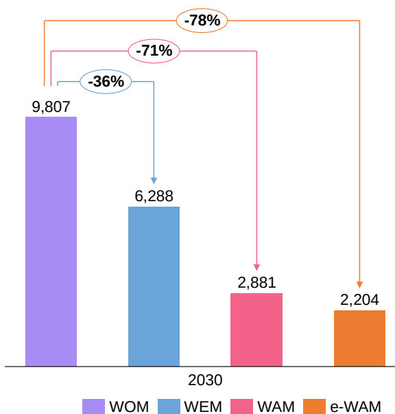
Figure 4-15: Comparison of total GHG emissions from all sectors without MEMO in WOM, WEM, WAM and e- WAM scenarios, 2030 (in Gg CO 2 -eq)
