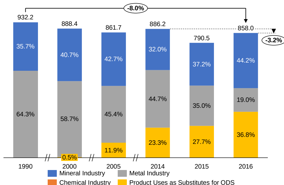
Figure 2-4: GHG emissions from the IPPU sector, by category (in Gg CO 2 -eq)
