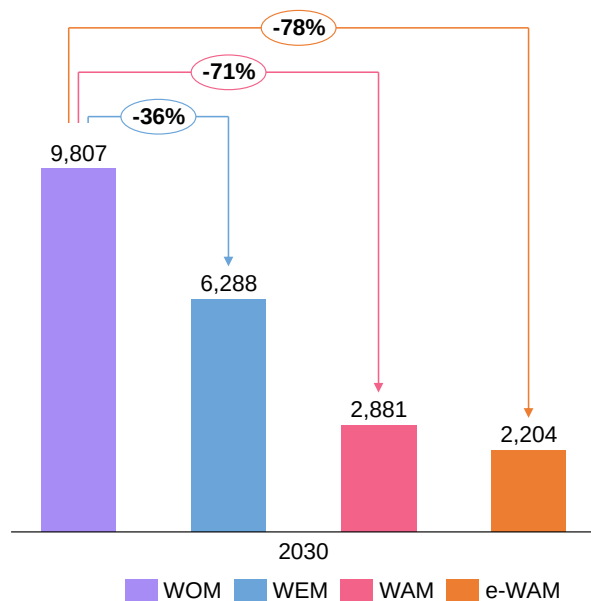
Figure 0-7: Comparison of total GHG emissions from all sectors without MEMO in WOM, WEM, WAM and e- WAM scenarios, 2030 (in Gg CO 2 -eq)
