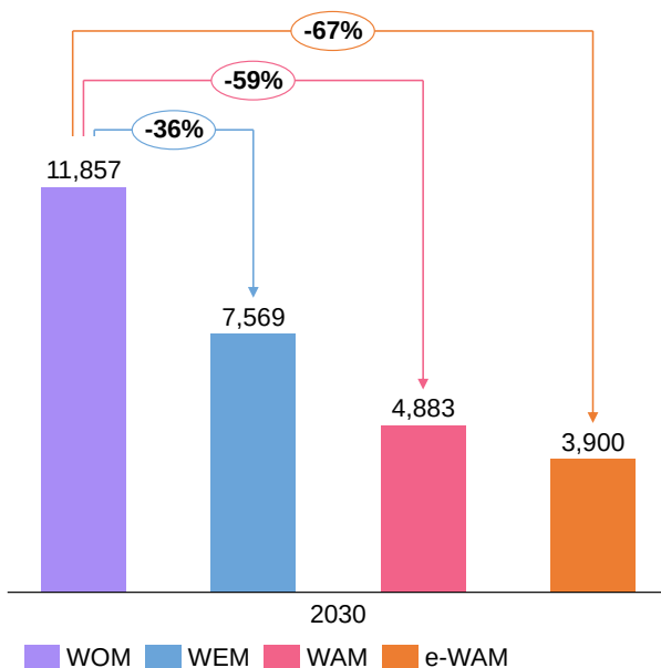
Figure 0-6: Comparison of total GHG emissions from all sectors in WOM, WEM, WAM and e- WAM scenarios, 2030 (in Gg CO 2 -eq)
