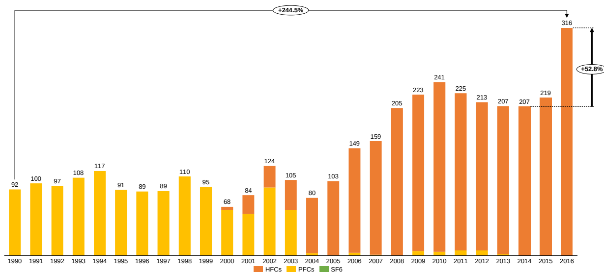
Figure 0-4: Emissions of F-gases (in Gg CO 2 -eq)
