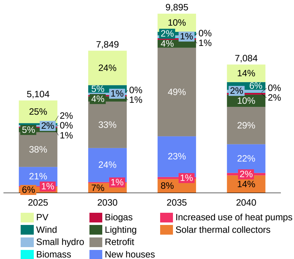
Figure 4-9: Number of domestic green jobs by technologies in E-WAM
