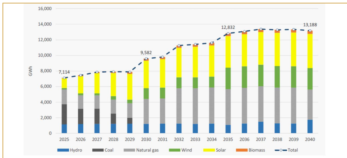
Figure 30 Electricity production, updated NECP
