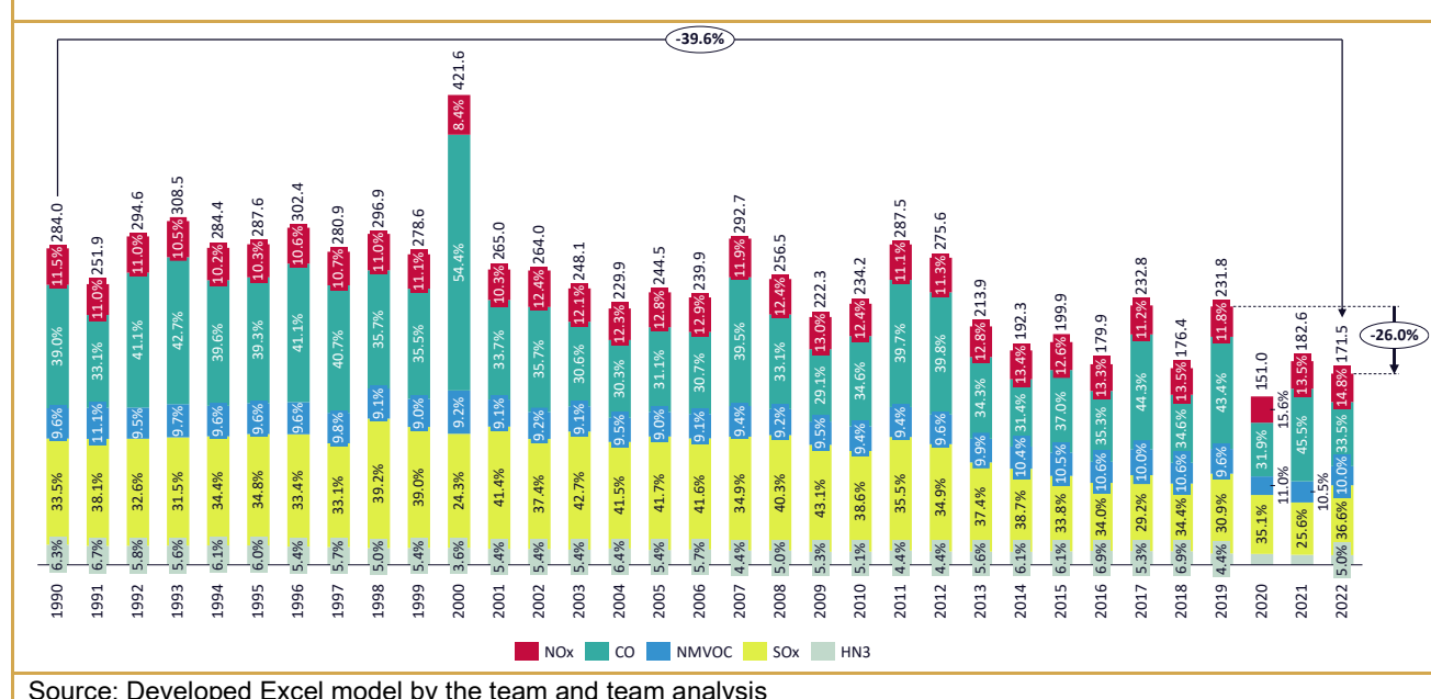
Figure 12. Emissions of NO x , CO, NMVOC, SO 2 and NH 3 in the period 1990 – 2022 (in Gg)
