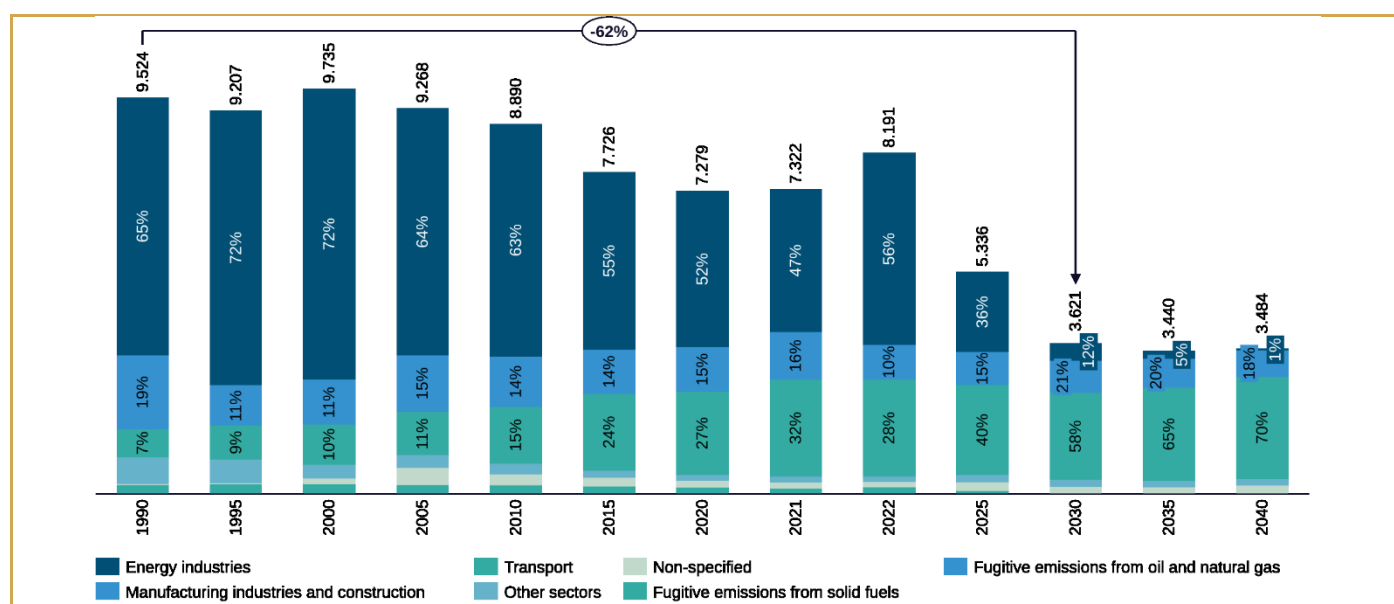
Figure 26 Total greenhouse gas emissions, Energy sector - WAM scenario (in Gg CO 2 -eq)
