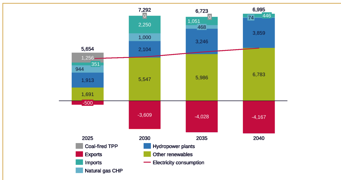
Figure 29 Electricity needs and supply, WAM scenario (in GWh)
