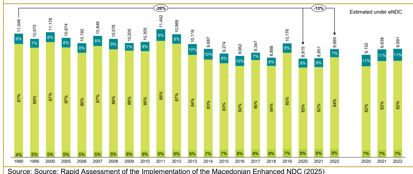
Figure 17. GHG emissions
